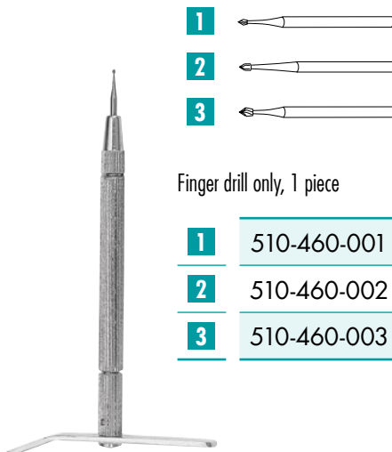
Finger nail drill complete with 3 drill points
